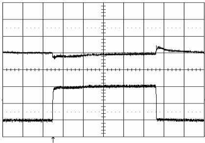
Output voltage response to load current step-change (5-15-5 A) at: T_{P1} = +25^{\circ}\text{C} , V_I = 12\text{ V} , C_O = 5\text{ mF} . Top trace: output voltage (200 mV/div.). Bottom trace: load current (10 A/div.). Time scale: (0.2 ms/div.).
