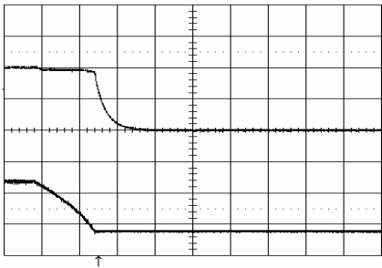
Shut-down enabled by disconnecting V_I at: T_{P1} = +25^{\circ}\text{C} , V_I = 12\text{ V} , I_O = 20\text{ A} resistive load. Top trace: output voltage (0.5 V/div.). Bottom trace: input voltage (5 V/div.). Time scale: (10 ms/div.).
