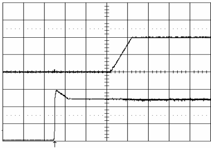
Start-up enabled by connecting V_I at: T_{P1} = +25^{\circ}\text{C} , V_I = 12\text{ V} , I_O = 20\text{ A} resistive load and 5\text{ mF} . Top trace: output voltage (0.5 V/div.). Bottom trace: input voltage (5 V/div.). Time scale: (10 ms/div.).
