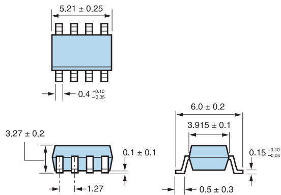
S08 1.27mm pin pitch
