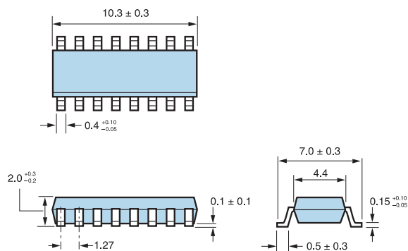
SSOP16 1.27mm pin pitch
