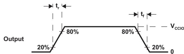
Figure 5-11. CMOS-Level Outputs
