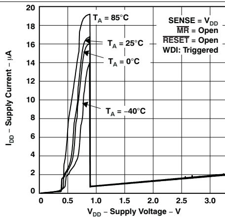
Figure 5. TPS3110E09 Supply Current vs Supply Voltage
