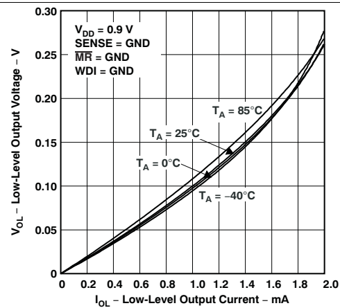
Figure 6. TPS3110E09 Low-Level Output Voltage vs Low-Level Output Current
