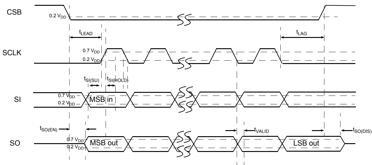
Figure 4. Timing Diagram
