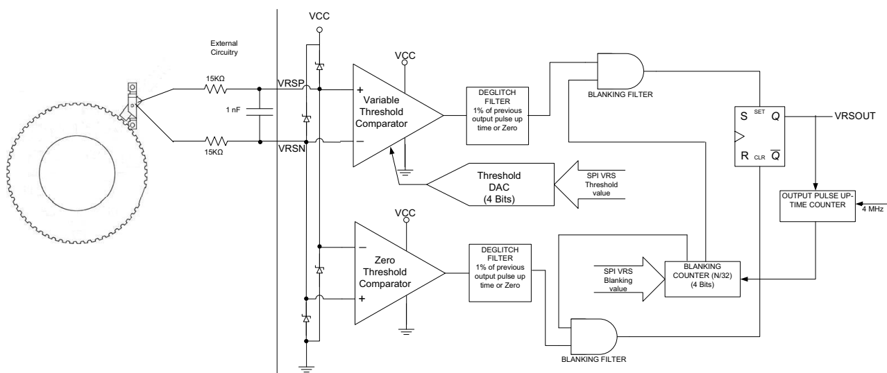
Figure 8. VRS Schematic
