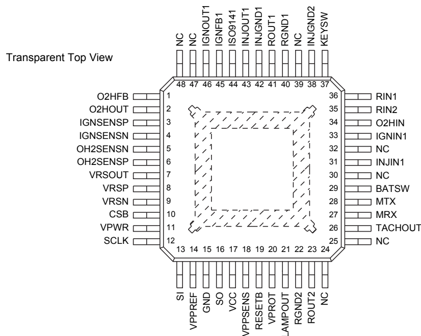
Figure 3. 33813 Pin Connections
