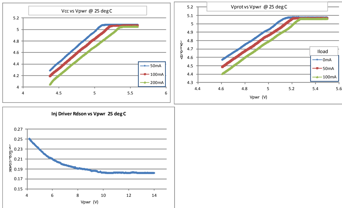
Figure 6. Typical Electrical Specifications
