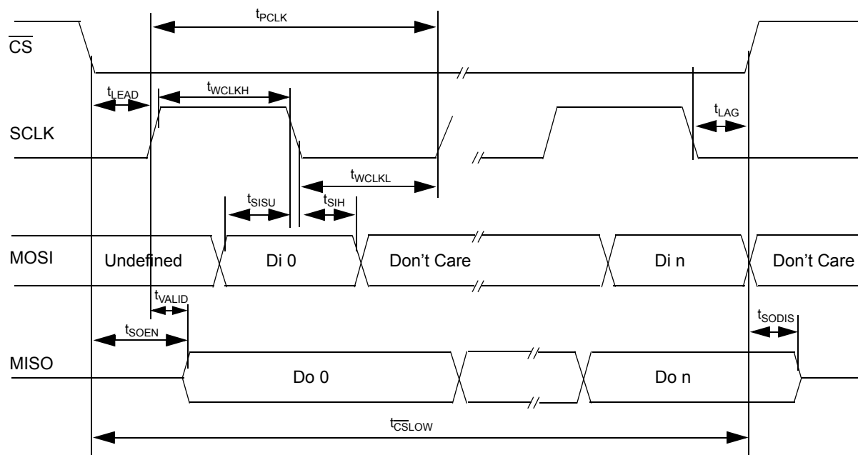
Figure 10. SPI Timings
