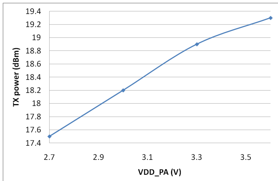
Figure 3: Typical TX power as a function of VDD_PA
