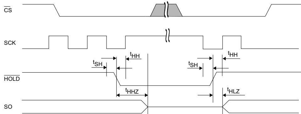
Figure 26. HOLD Timing
