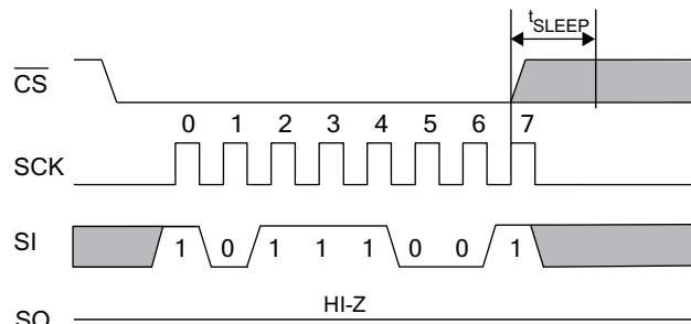
Figure 19. Sleep Mode Entry
