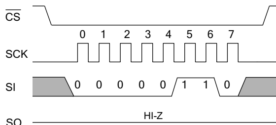
Figure 9. WREN Instruction
