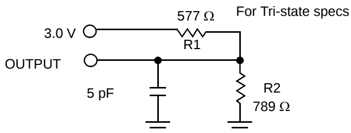
Figure 24. AC Test Loads and Waveforms
