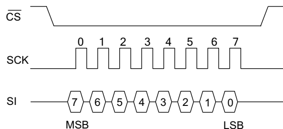
Figure 5. SPI Mode 0
