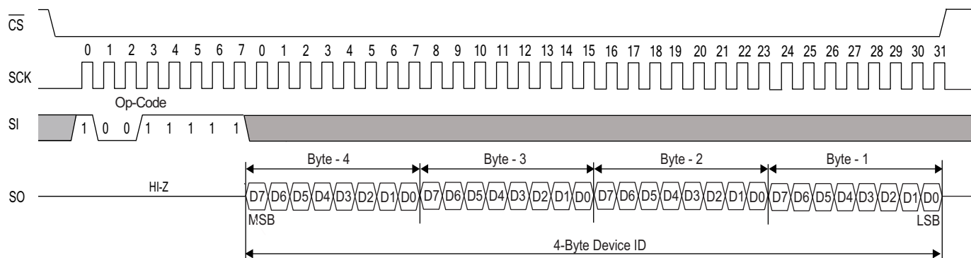
Figure 22. RDID instruction
