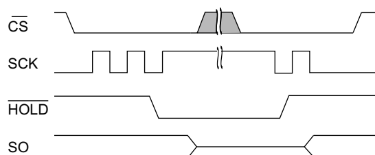
Figure 23. \overline{HOLD} Operation
