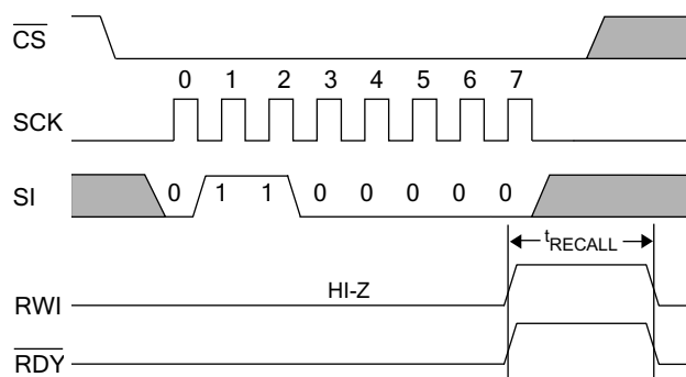
Figure 29. Software RECALL Cycle [18]
