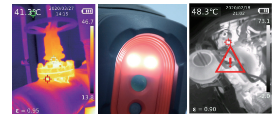
Center/highest/lowest temperature point LED alarm Image alarm
