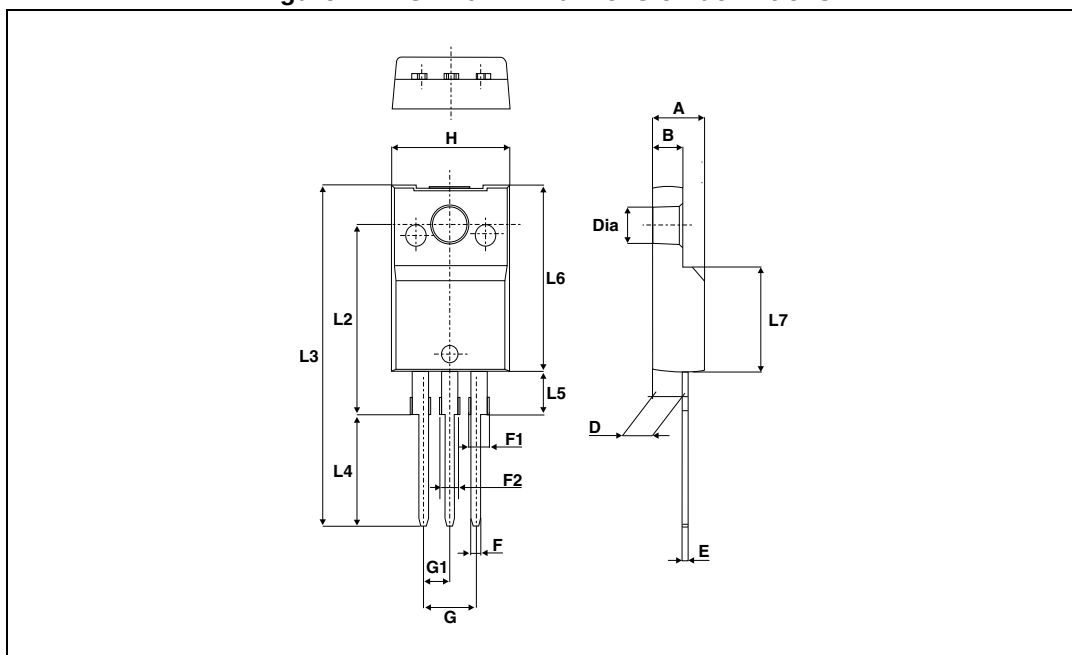
Figure 14. TO-220FPAB dimension definitions
