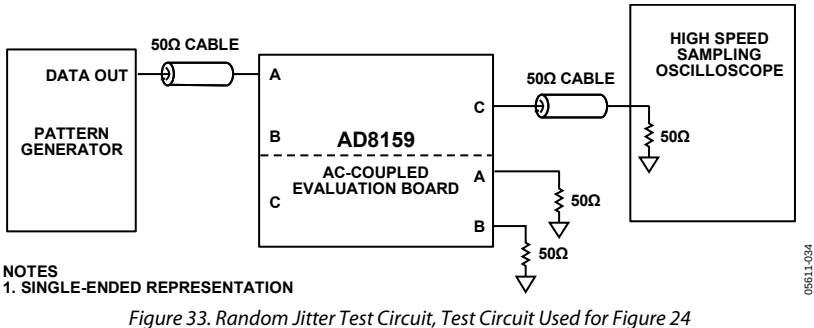
Figure 33. Random Jitter Test Circuit, Test Circuit Used for Figure 24
