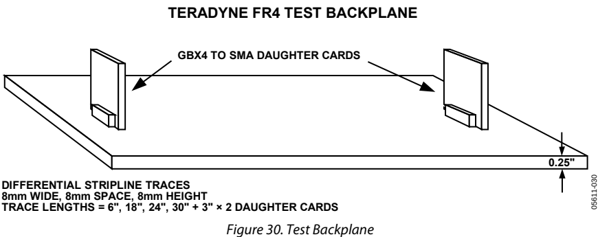
Figure 30. Test Backplane
