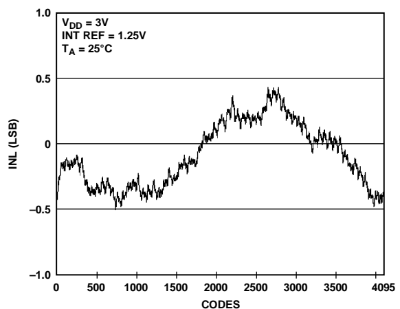
Figure 21. INL AD5628-1
