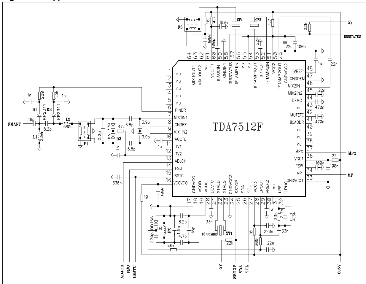
Figure 9. Application circuit
