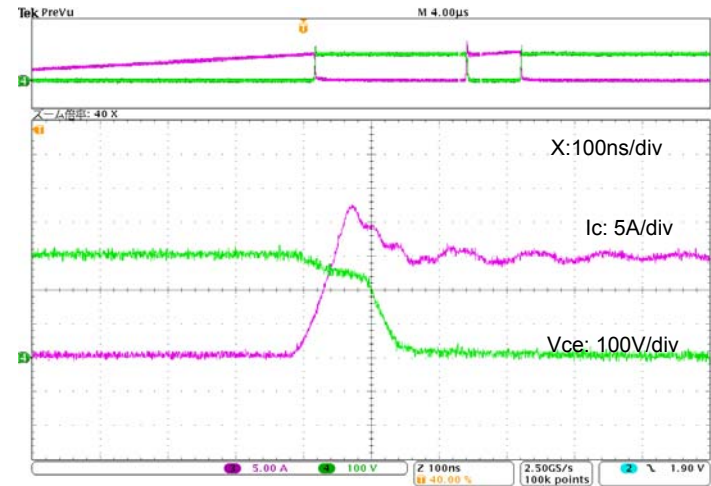
Fig. 13 IGBT Turn-on. Typical turn-on waveform at T_c=100^{\circ}C , V_{cc}=300V , I_c=15A
