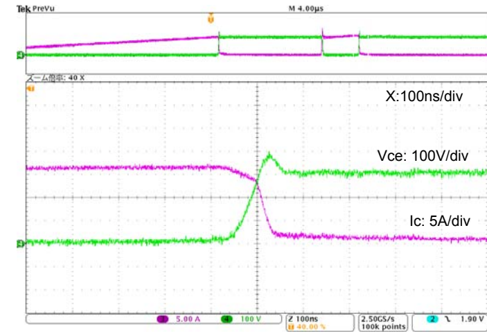
Fig. 14 IGBT Turn-off. Typical turn-off waveform T_c=100^{\circ}C , V_{cc}=300V , I_c=15A
