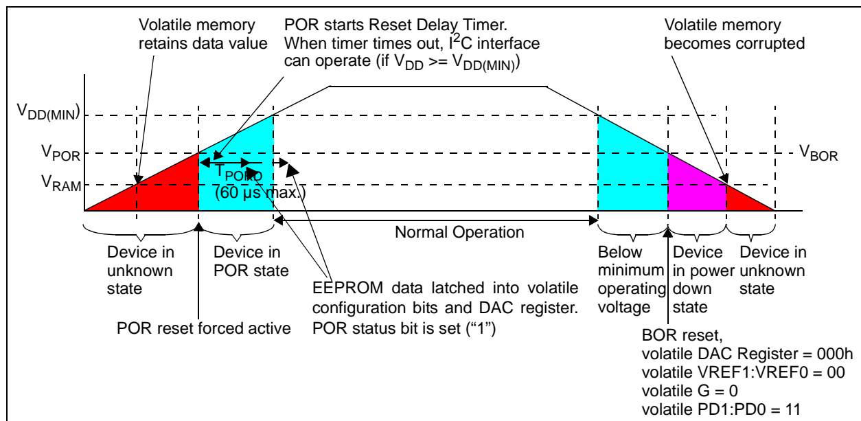
FIGURE 4-1: Power-On-Reset Operation.
