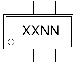
6-Lead SOT-23
