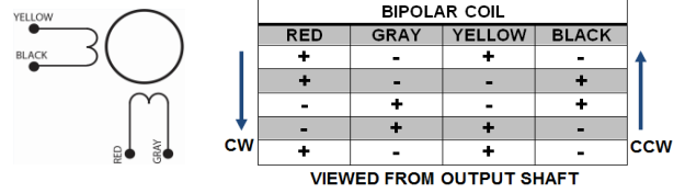
VIEWED FROM OUTPUT SHAFT
