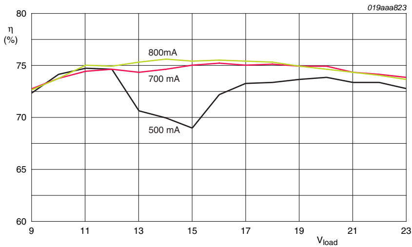
Fig 14. 230 V (AC) efficiency curve
