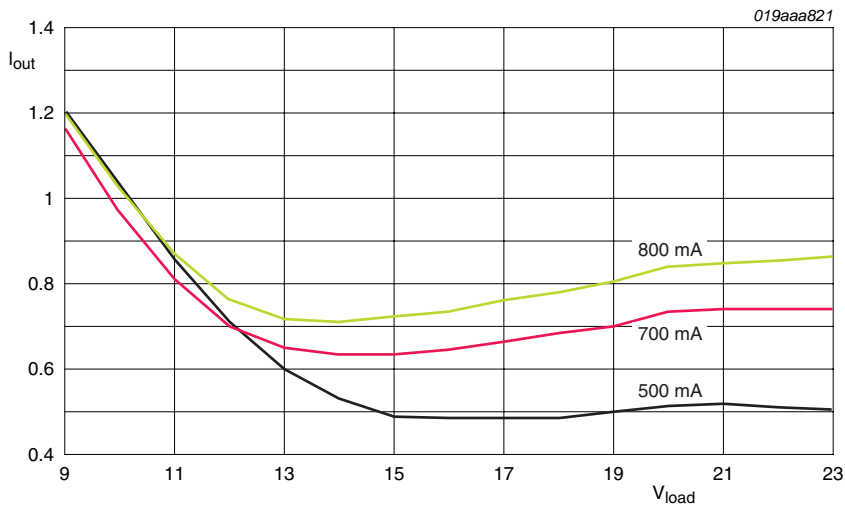
Fig 12. 230 V (AC) load curve
