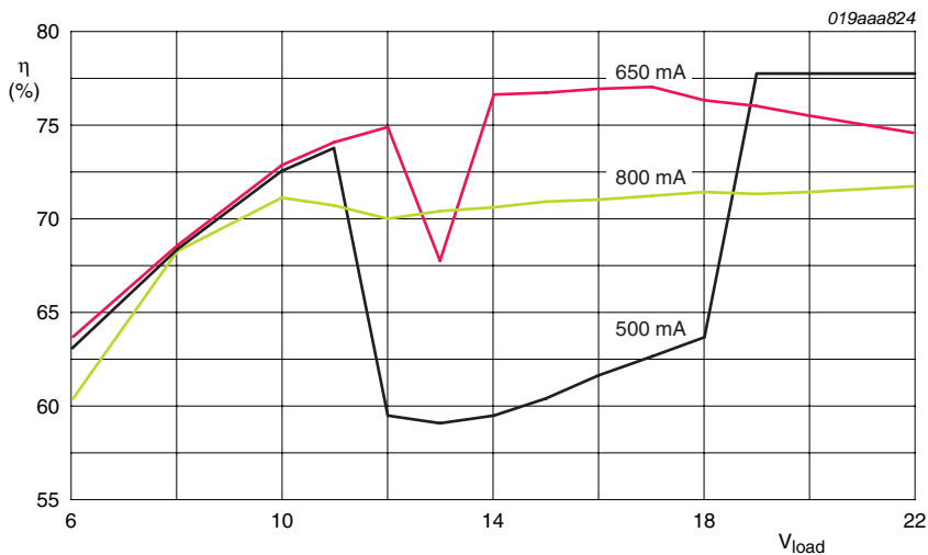
Fig 13. 120 V (AC) efficiency curve
