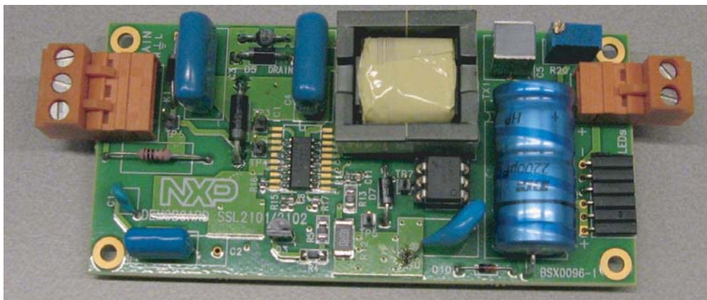
Fig 3. Demo board (top)
