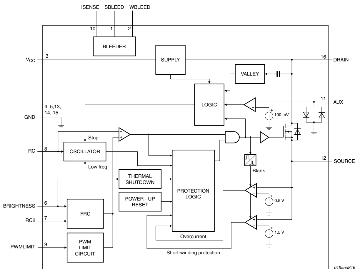
Fig 5. Block diagram SSL2101
