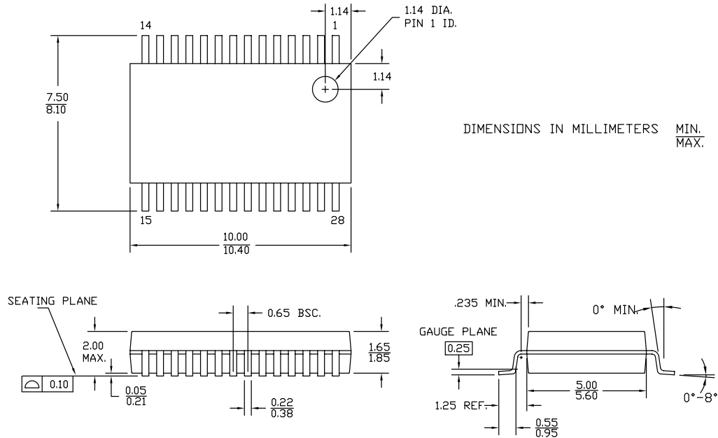
Figure 13. 28-pin SSOP (210 Mils) O28.21 Package Outline, 51-85079
