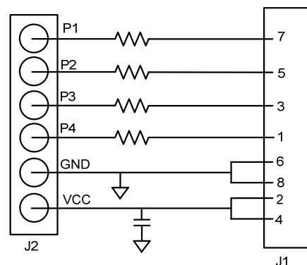
PmodRJ45 (Male) Circuit Diagram
