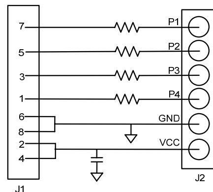
PmodRJ45 (Female) Circuit Diagram
