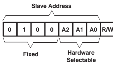
Figure 18. TCA9554 Address
