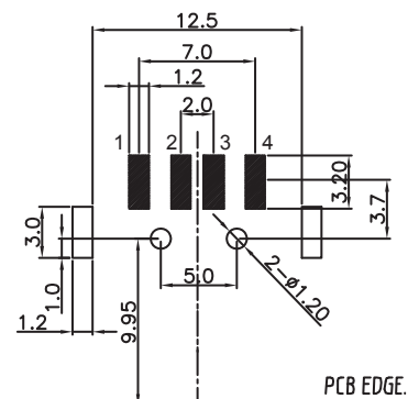
PCB LAYOUT - COMPONENT VIEW PCB THICKNESS 1.60 MM
