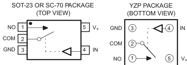
Pin Functions
