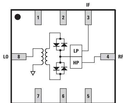
Figure 11. Simplified schematic of the mixer
