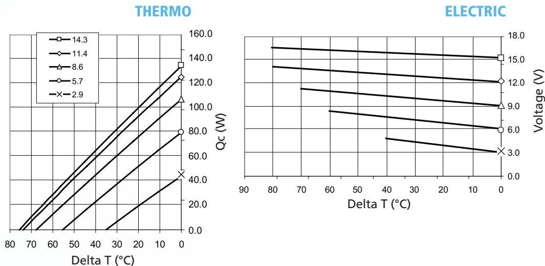
Performance Curves at T_h = 50^\circ\text{C}
