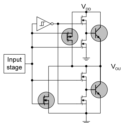
Figure 31. MillerDrive™ Output Architecture
