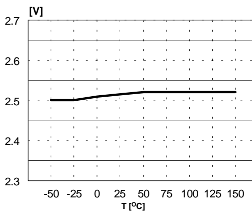
Figure 12. ACsense reference
