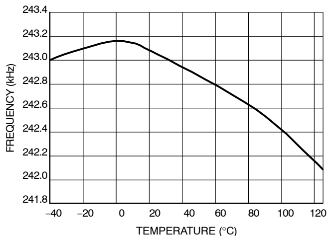
Figure 9. F swmax
