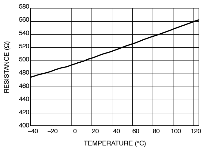
Figure 13. R t_discharge
