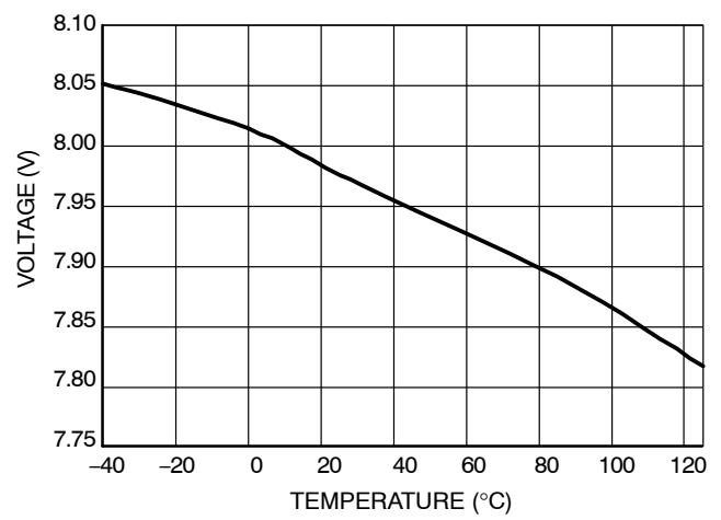
Figure 6. V BOOTmin
