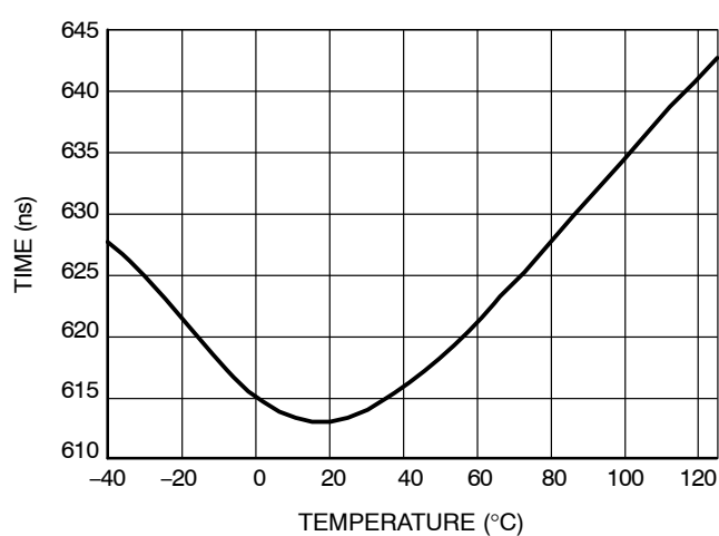
Figure 14. T dead
