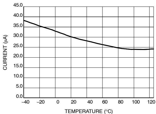
Figure 11. I cc_startup
