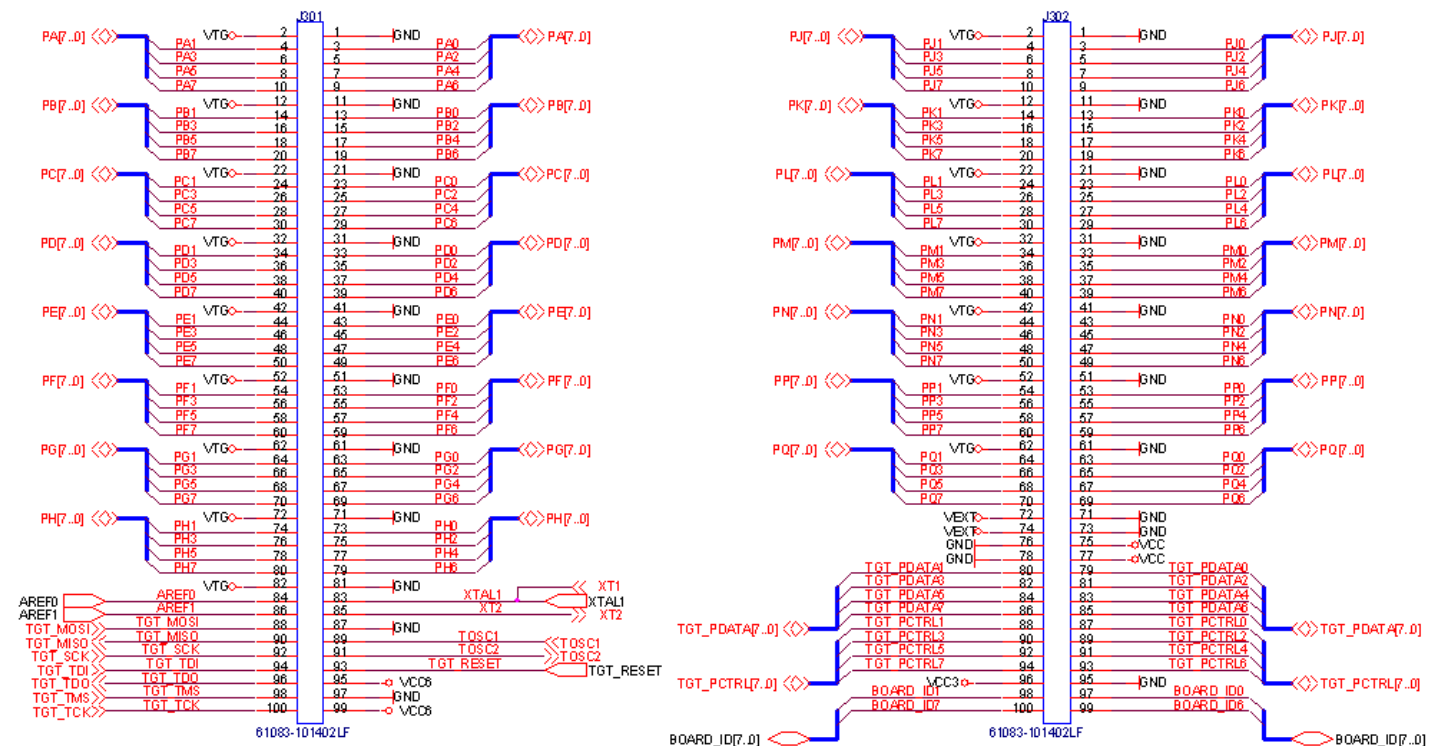
Figure 3-2. Pinout for expansion connectors.
