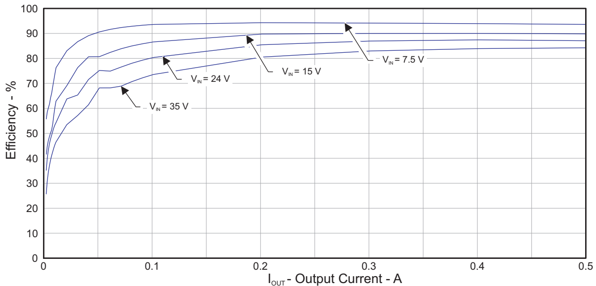
Figure 1. TPS5401EVM-708 Efficiency
