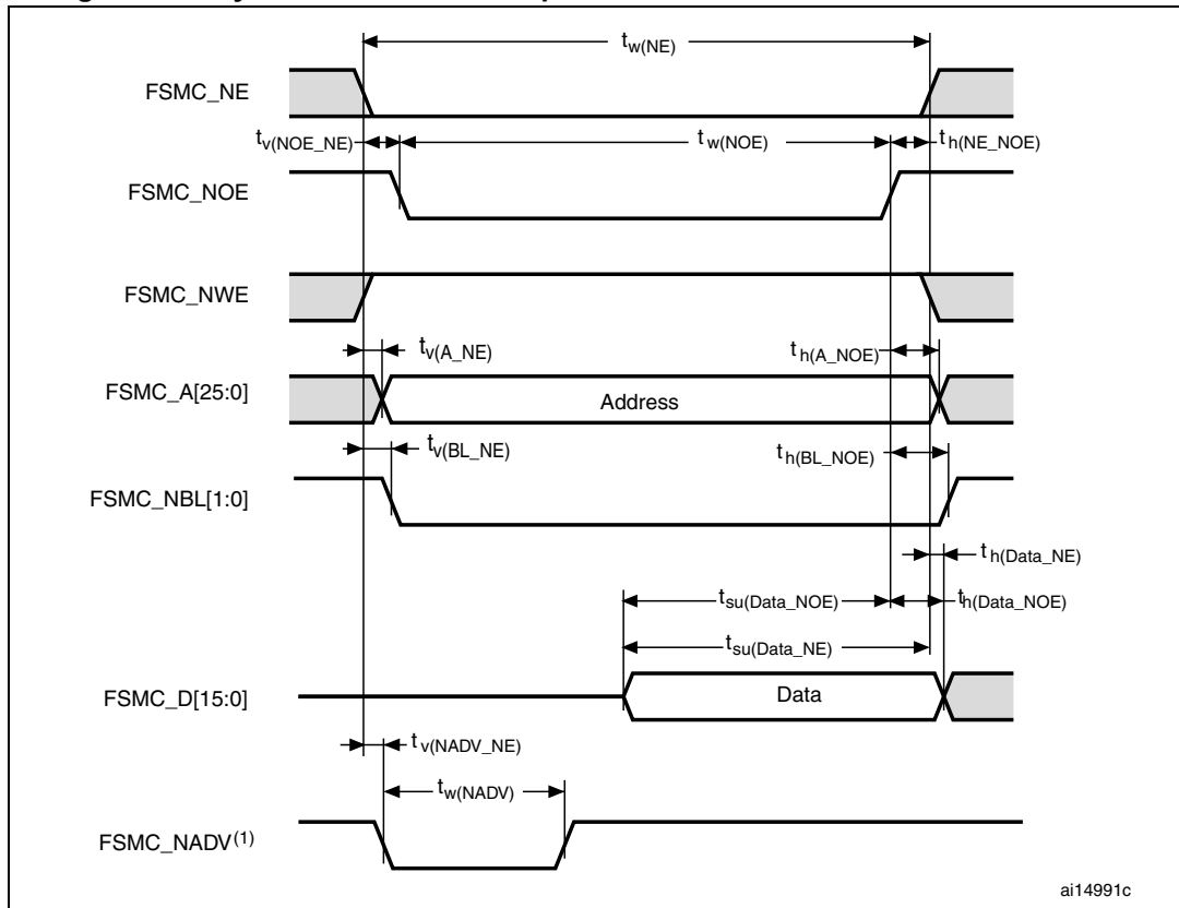
Figure 57. Asynchronous non-multiplexed SRAM/PSRAM/NOR read waveforms
