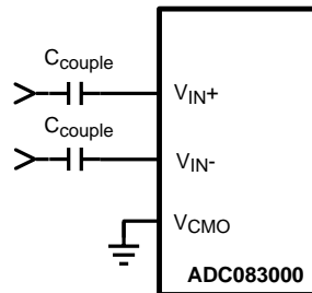
Figure 36. Differential Data Input Connection
