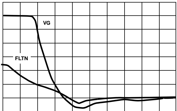
VOLTAGE (2V/DIV) TIME (2μs/DIV) FLTN = 0.01μF
