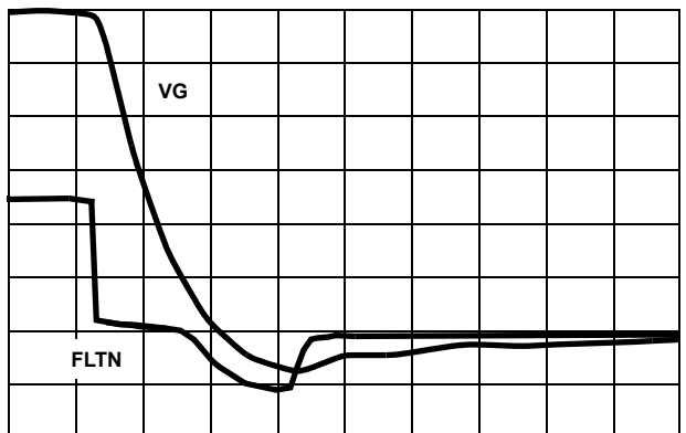
VOLTAGE (2V/DIV) TIME (1μs/DIV) FLTN = OPEN
