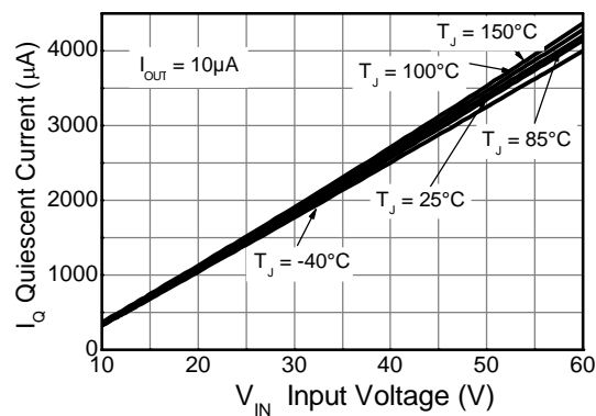
Quiescent Current
