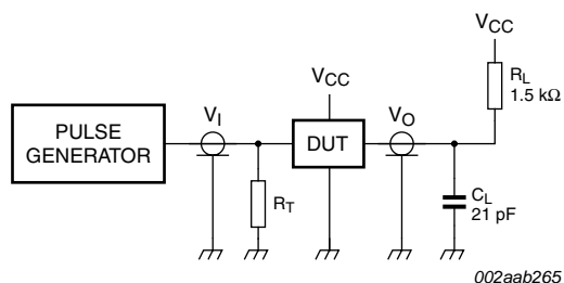
Fig 13. Load circuit for open-drain LVTTTL I/O and open-drain outputs
