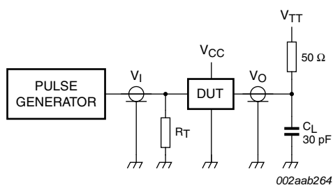
Fig 12. Load circuit for B outputs
