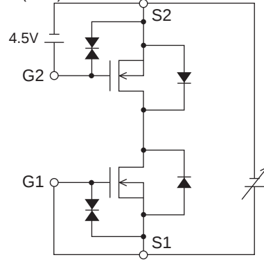
Test Circuit 6
