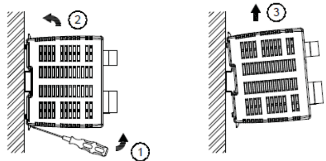
Fig. 2.2 Dismounting
