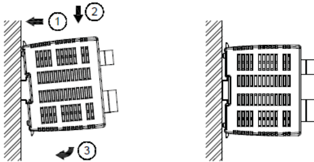
Fig. 2.1 Mounting
