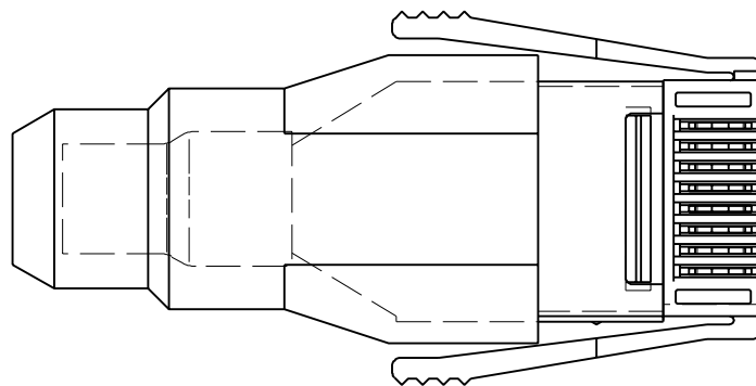
KEYING OPTION "2"
