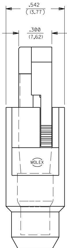
TERMINATED VIEWS
