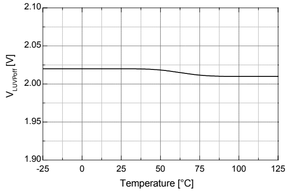
Figure 16. LUVF On-to-Off Voltage vs. Temp.
