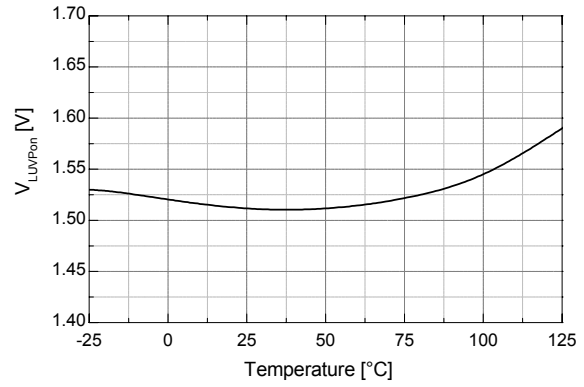
Figure 17. LUVF Off-to-On Voltage vs. Temp.
