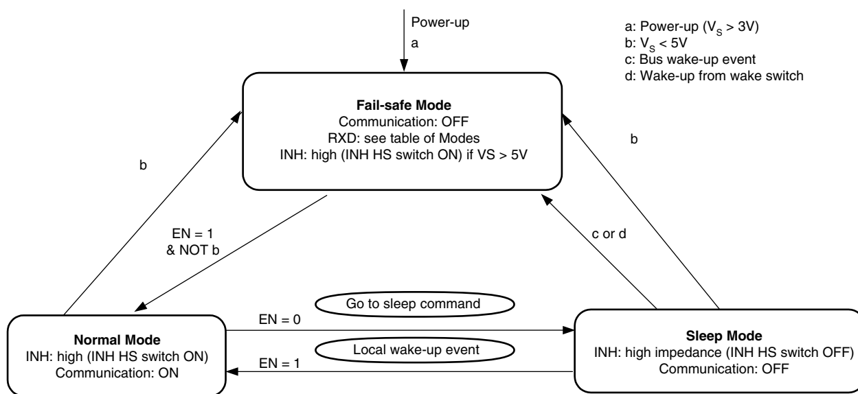
Figure 2-1. Modes of Operation
