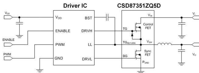
TYPICAL CIRCUIT
