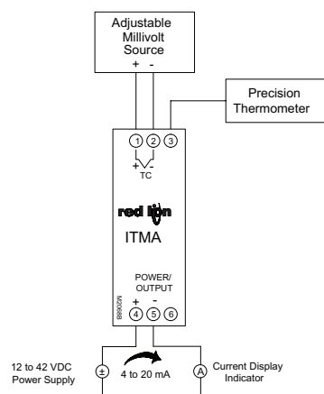
Ice Point Calibration Wiring
