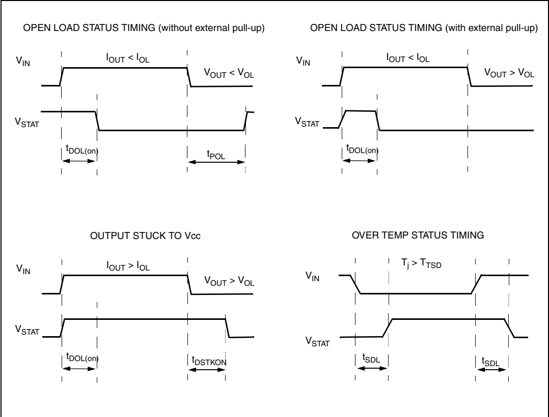
Figure 4. Status timings
