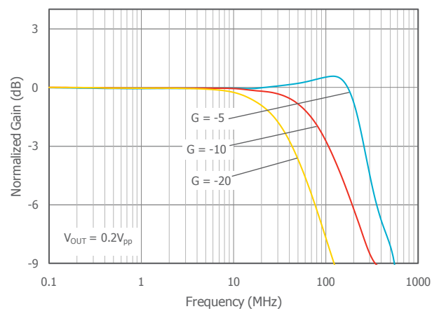
Inverting Frequency Response at V_S = 5\text{V}
