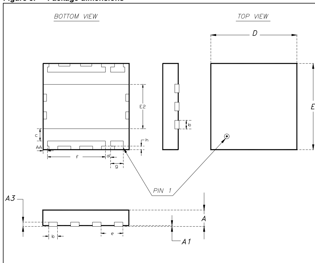
Figure 6. Package dimensions
