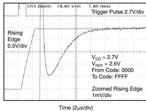
FULL-SCALE SETTLING TIME: 2.7V RISING EDGE
