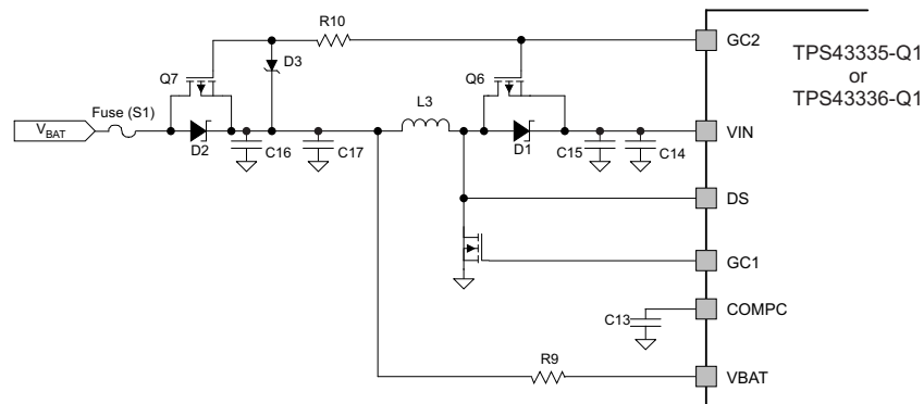
Figure 24. Reverse Battery Protection Option 1 for Buck Boost Configuration
