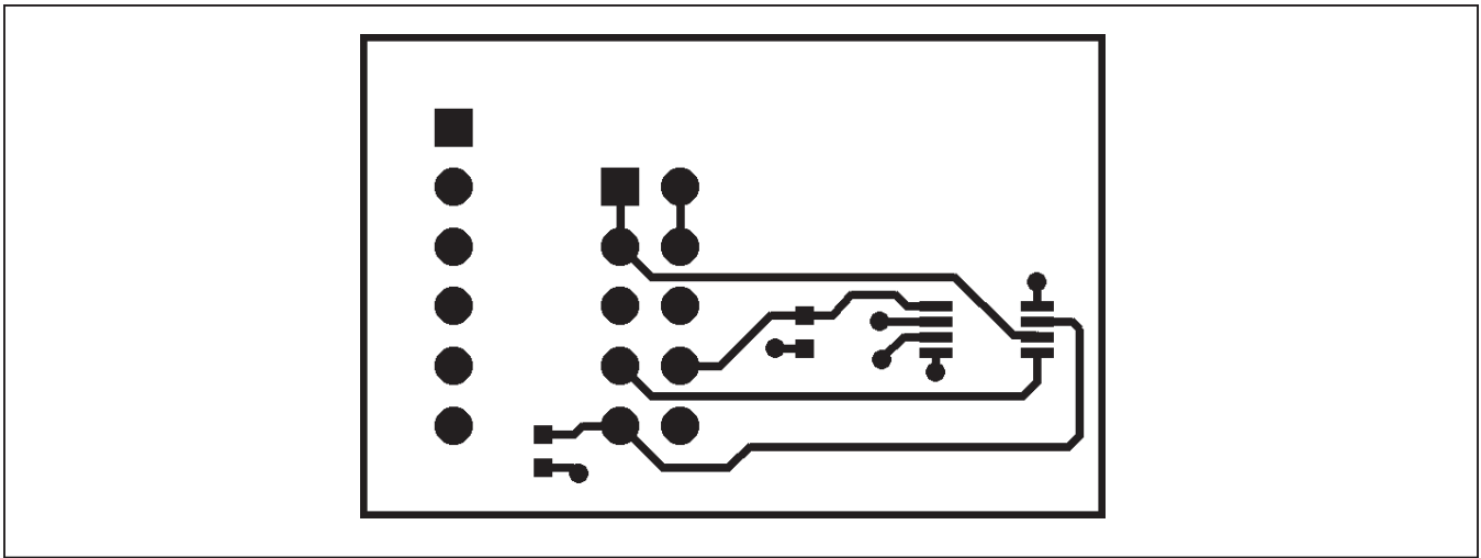
Figure 4. MAX31723PMB1 Peripheral Module PCB Layout—Component Side
