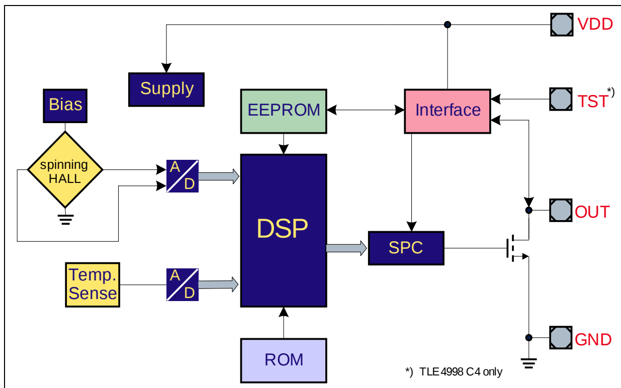
Figure 3 Block diagramm
