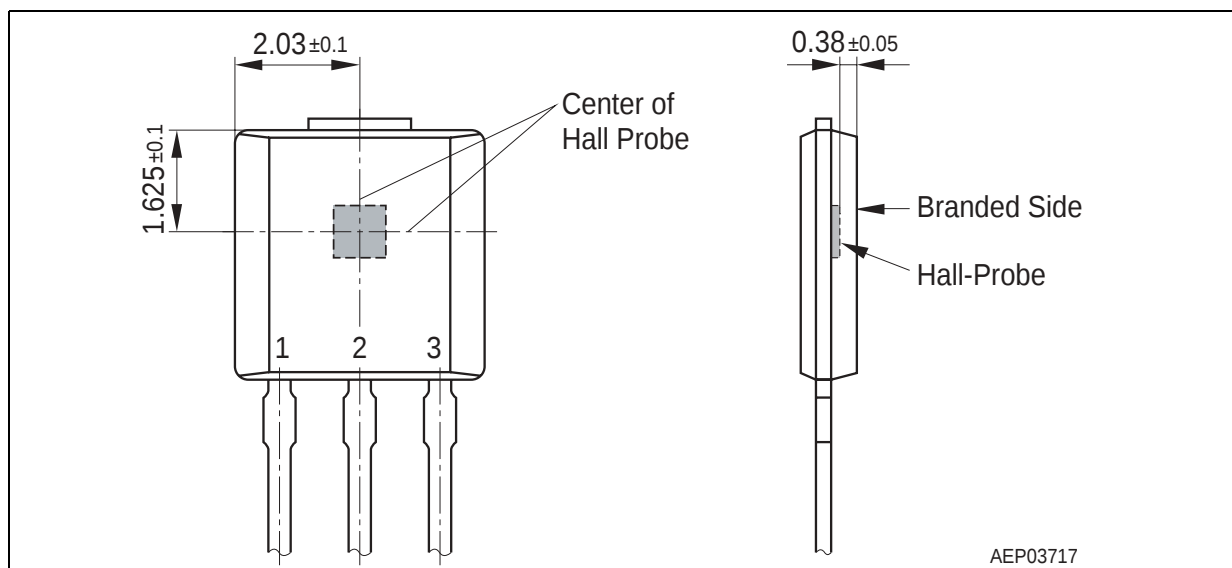
Figure 1 Hall Cell Location and Pin Configuration of PG-SSO-3-10 package
