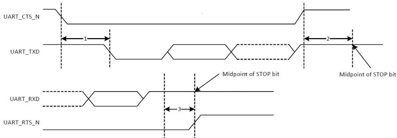
Figure 5 UART Timing
