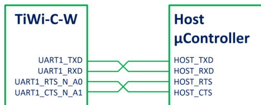
Figure 4 UART Connection from TiWi-C-W to Host
