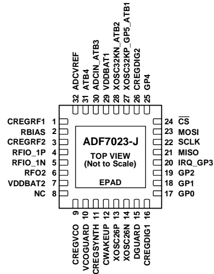
Figure 4. Pin Configuration
