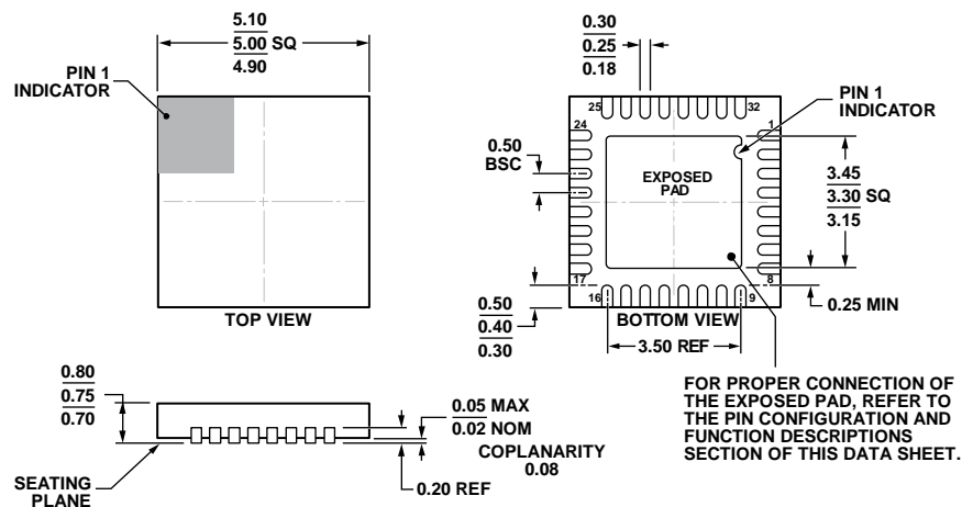
Figure 89. 32-Lead Lead Frame Chip Scale Package [LFCSP_WQ] 5 mm x 5 mm Body, Very Very Thin Quad (CP-32-13) Dimensions shown in millimeters
